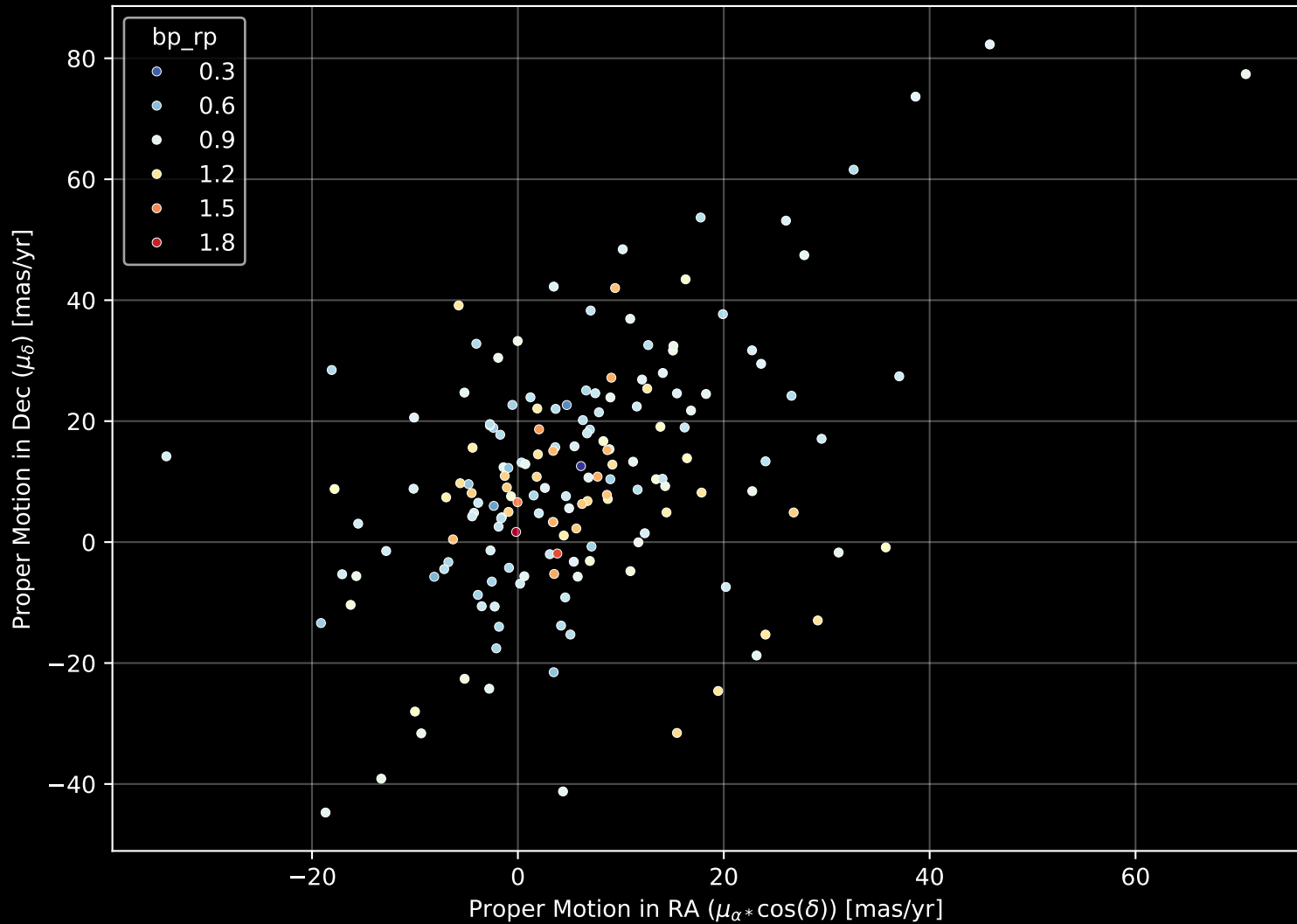
GALAH DR4 Field: [7205] Proper Motion Diagram (n= 167)
