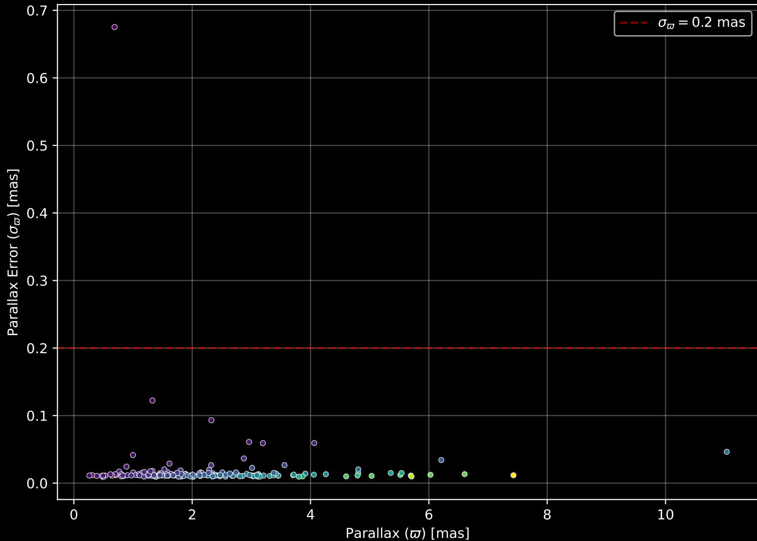
GALAH DR4 Field: [7205] Parallax Quality (n= 167)
