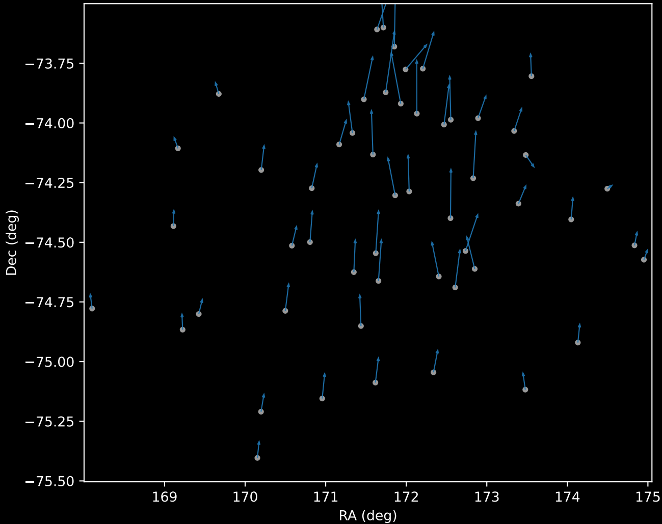
GALAH DR4 Cluster 0 Proper Motion Vectors (n=53)
