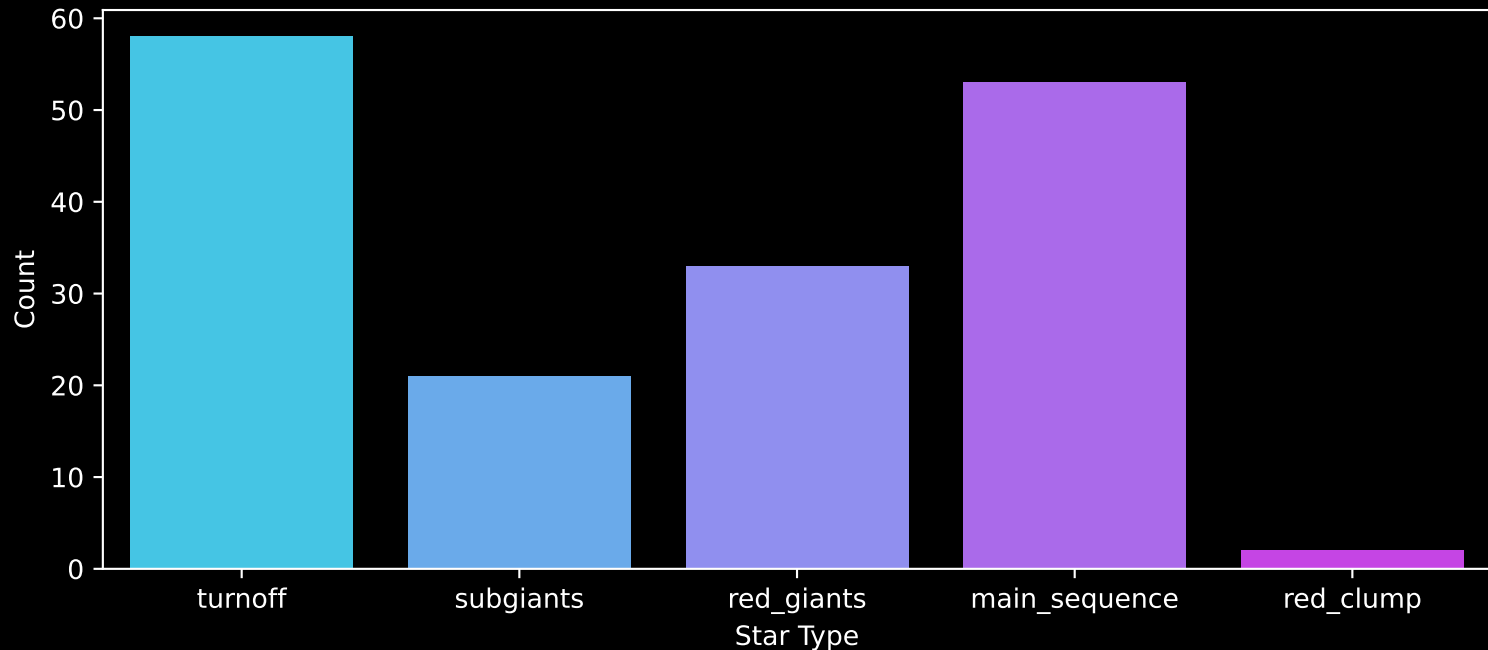
GALAH DR4 Field: [7205] Count plot of Star Type
