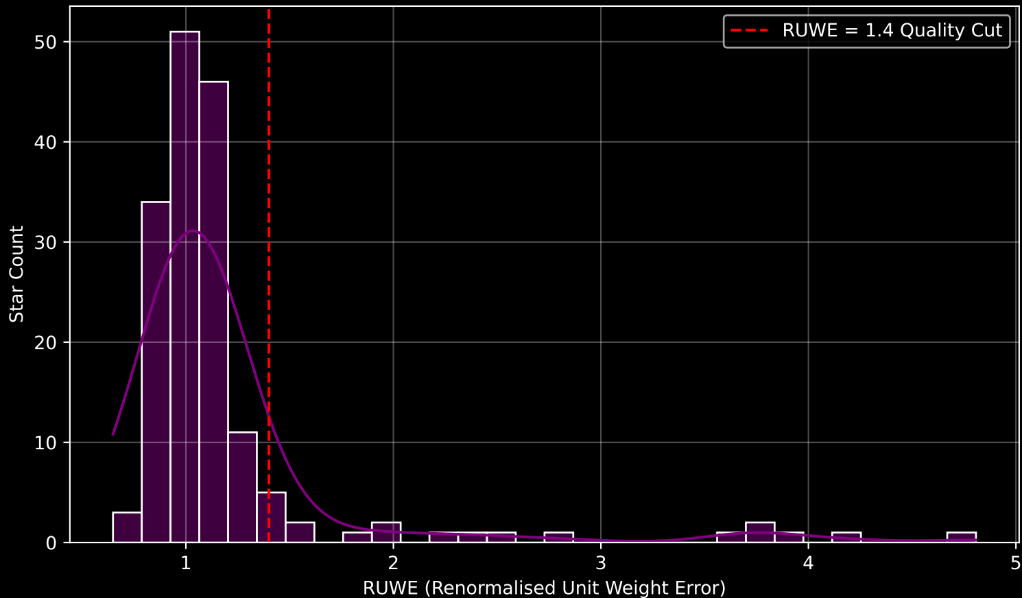
GALAH DR4 Field [7205] RUWE Distribution (n= 165)
